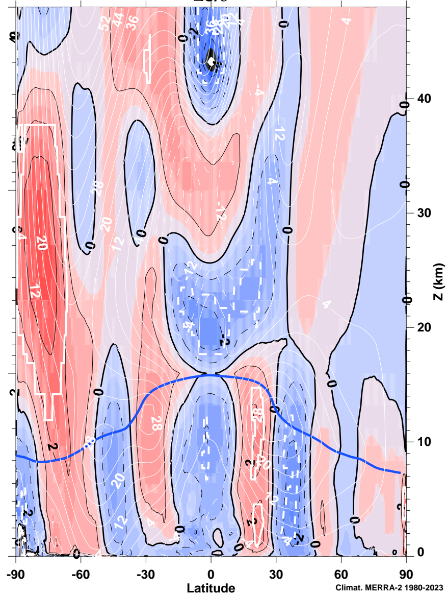
\Delta U/\sigma
