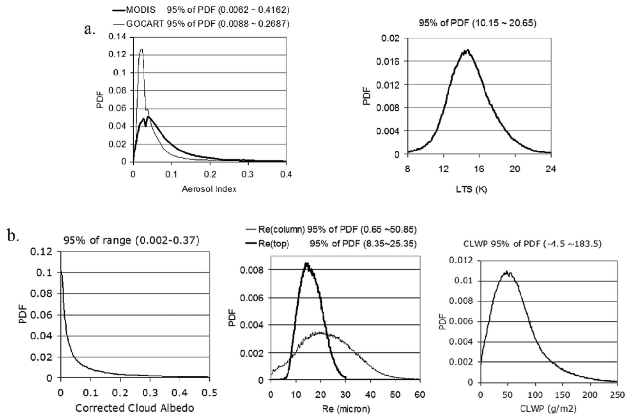
Figure 3. Probability density function (PDF) of (a) AI and LTS and (b) cloud properties. Variability of 95% of the total PDF is shown for each variable.
