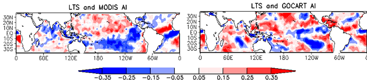
Figure 7. Linear correlation coefficient between AI and LTS in each 4^\circ box on a global grid for the same annual sampling period as in Figure 6. Positive AI-LTS (red) correlations mean that high AI appears with high LTS, while negative AI-LTS correlations mean that high AI appears with low LTS, which has opposite effect on cloud properties. Therefore negative-correlation regions appear to be coherent with the weak-correlation regions in Figure 6.
