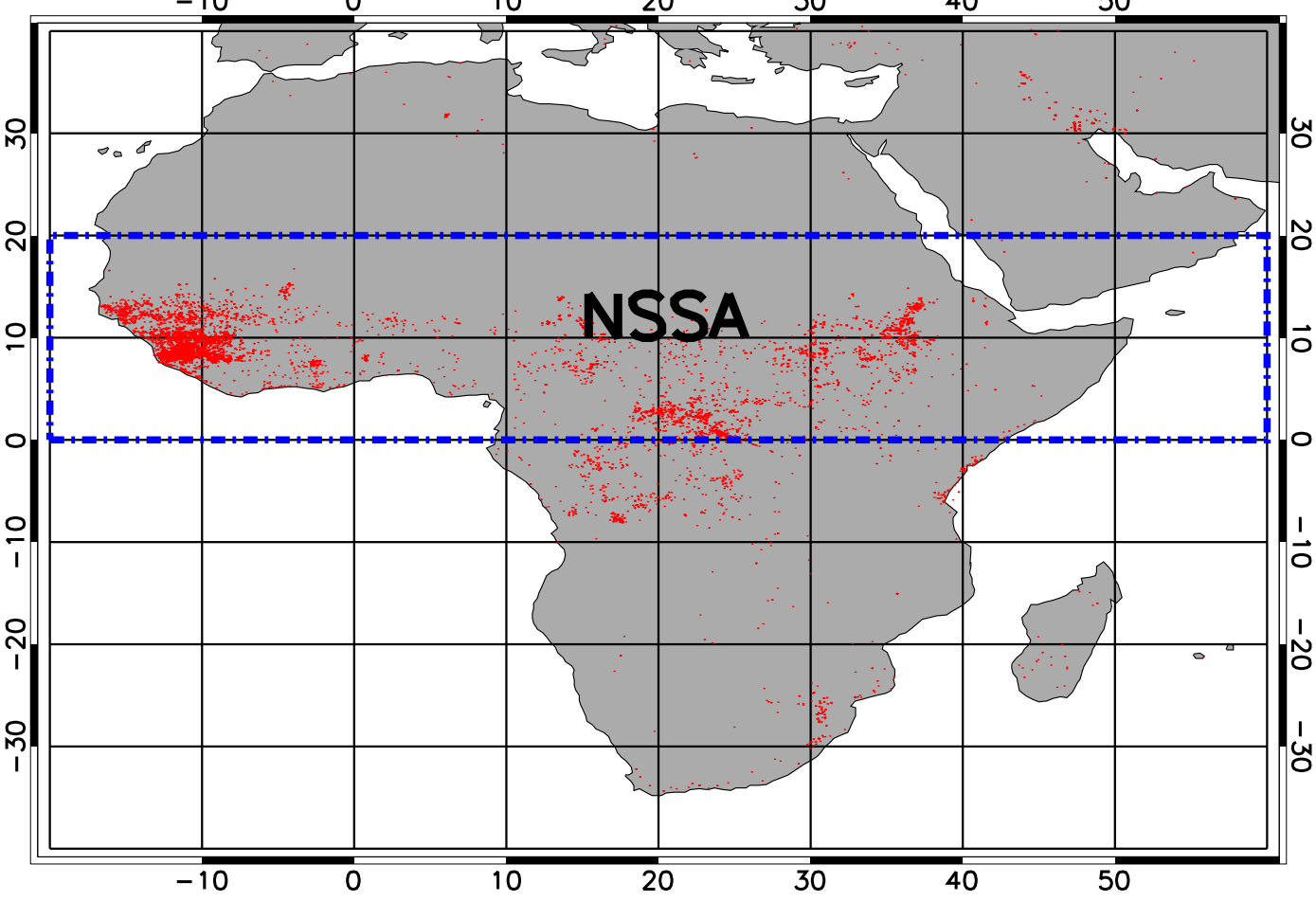
MODIS fire hotspots since Apr 1 to Apr 4 2016
